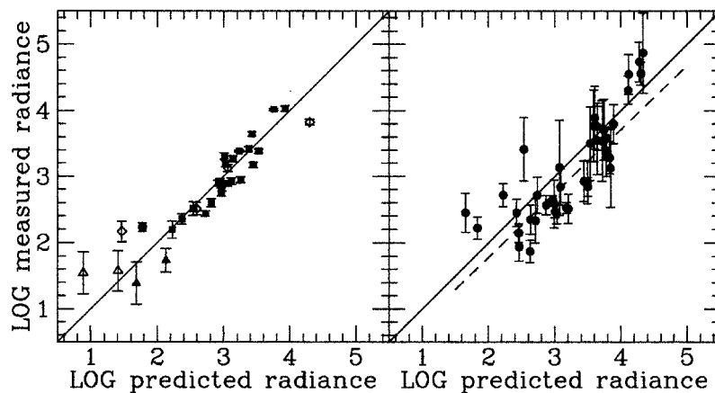
Figure 10. Comparison between map predictions and measurements of artificial night sky brightness measurements at the bottom of the atmosphere taken in clean or photometric nights in the V band in Europe (filled squares), North America (open triangles), South America (open rhombi), Africa (filled triangles) and Asia (filled circle). Right panel: map predictions versus photographic measurements taken in Japan in the period 1987–1991 with variable atmospheric aerosol content and averaged for each site. The large error bars show the effects of the changes in the atmospheric aerosol content and in the extinction of the light of the comparison star. The dashed line shows the linear regression. Night sky brightnesses are expressed as photon radiances.
